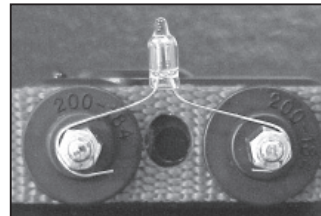
Test Light on Receiver Contact Points
